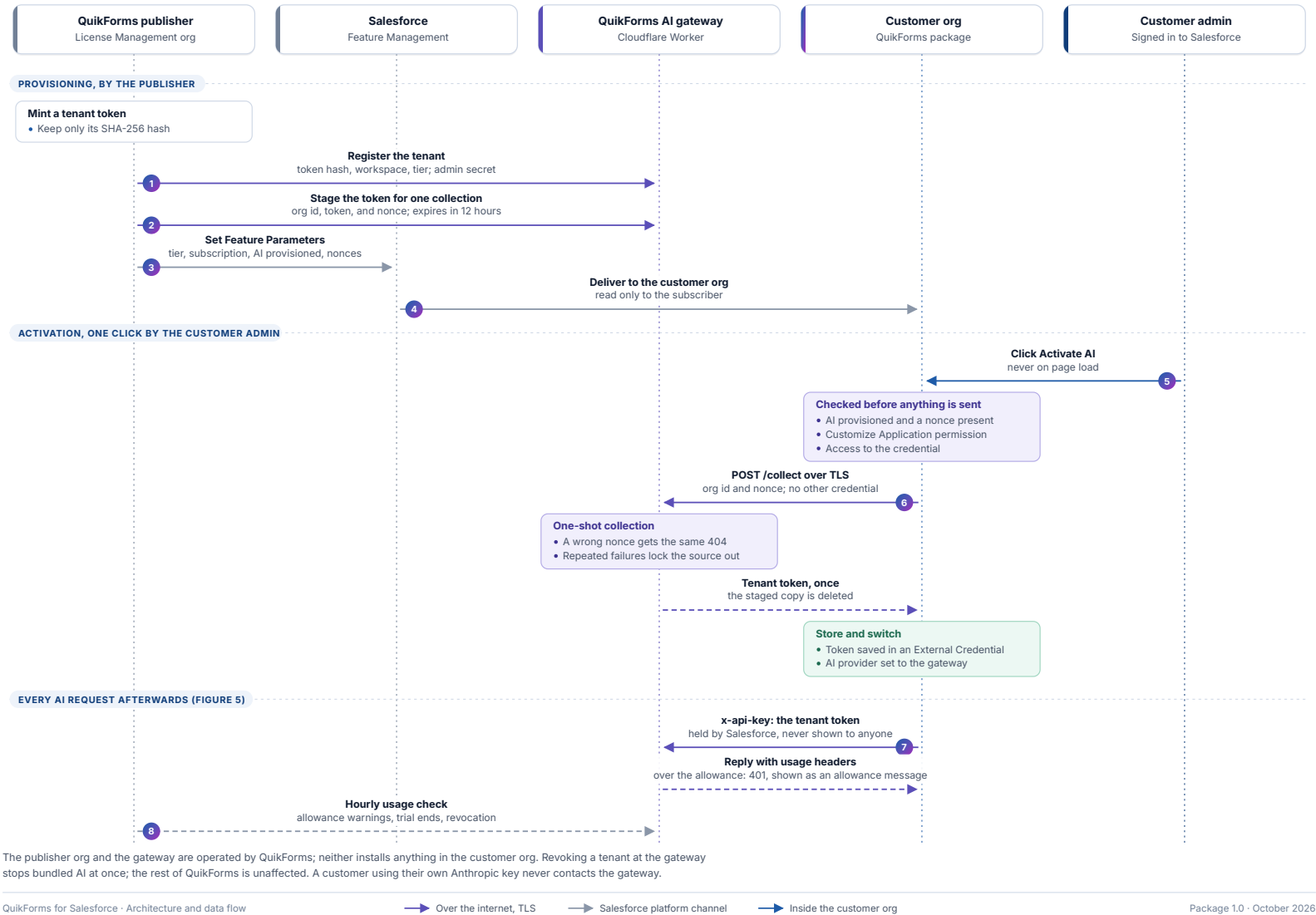
Figure 6. License flags arrive as Feature Parameters; the bundled AI token is collected once, on an admin's click.
