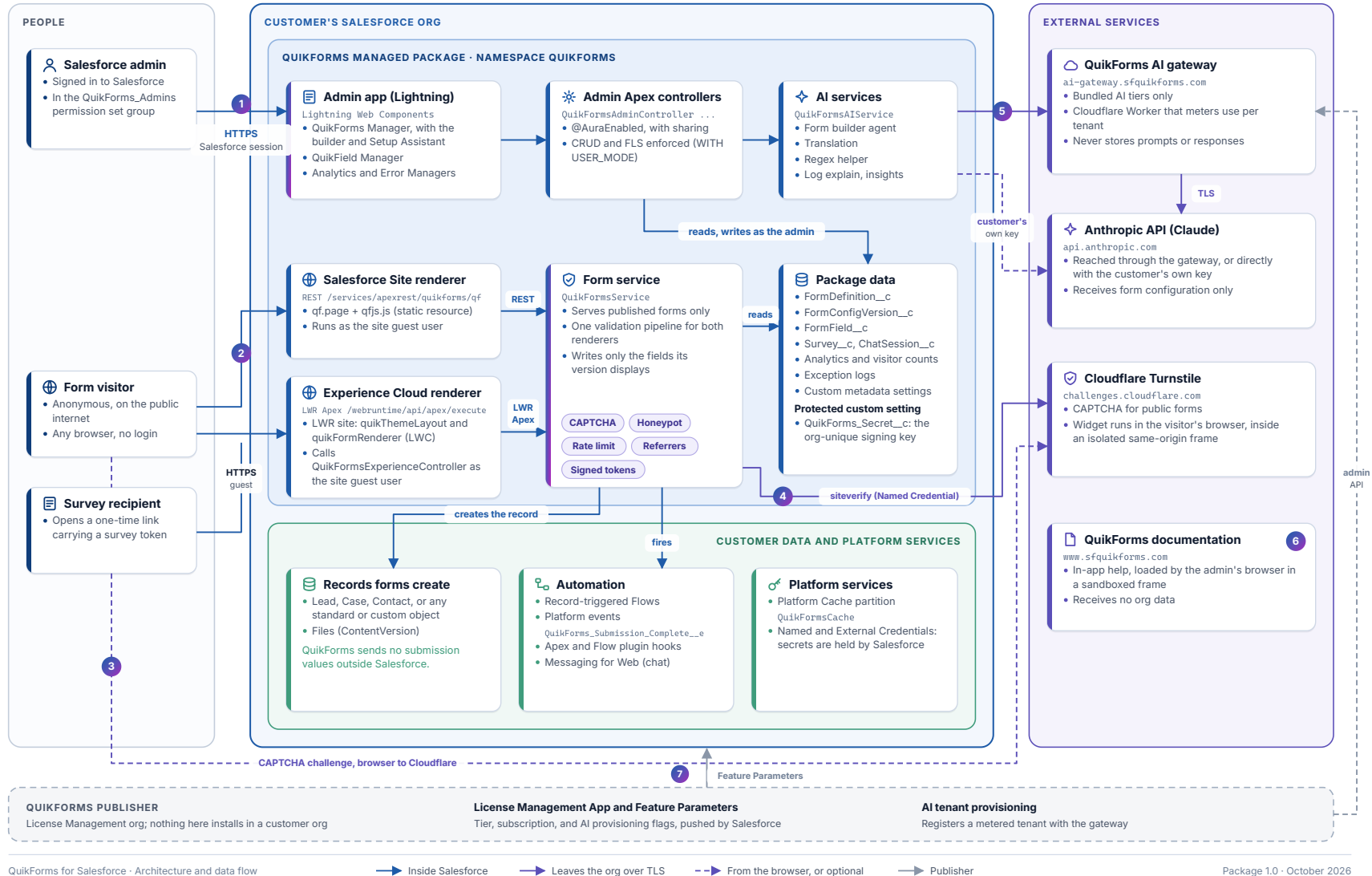
Figure 2. These are the components and their trust boundaries. Numbered connections are described in Authentication at each boundary .
