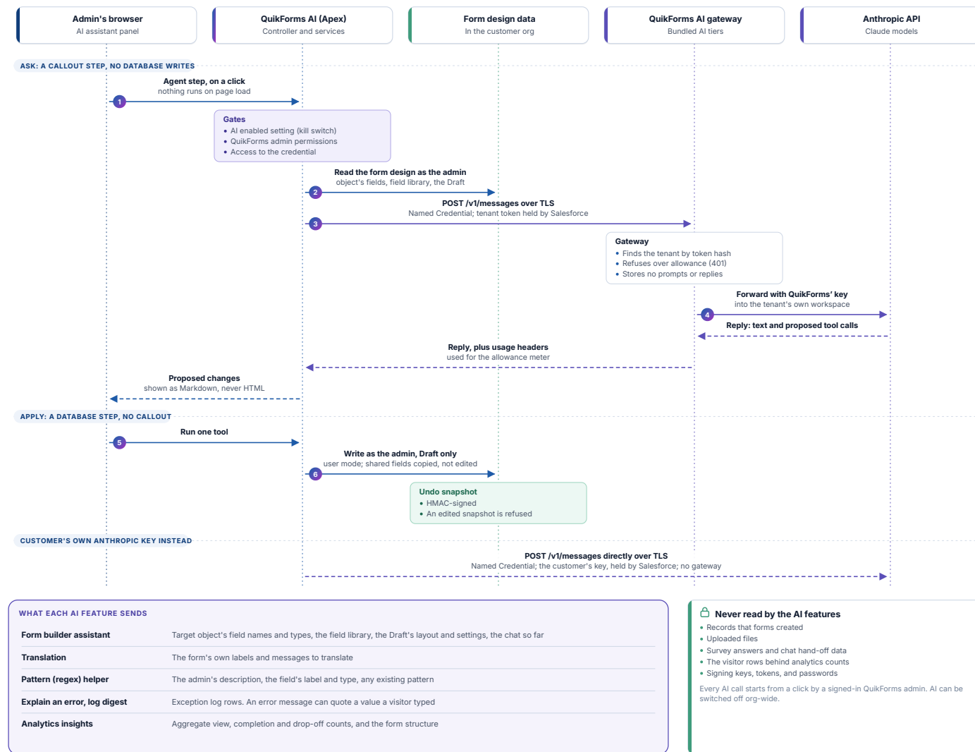
Figure 5. AI is admin-only, started by a click, and can be switched off for the whole org.
